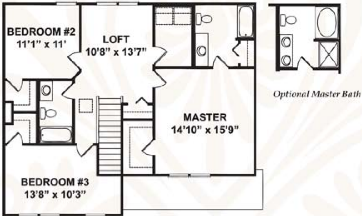
Second Floor
